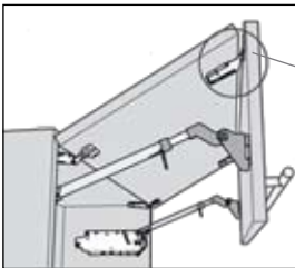
Verbindingscharnier Hinge between 2 front parts
